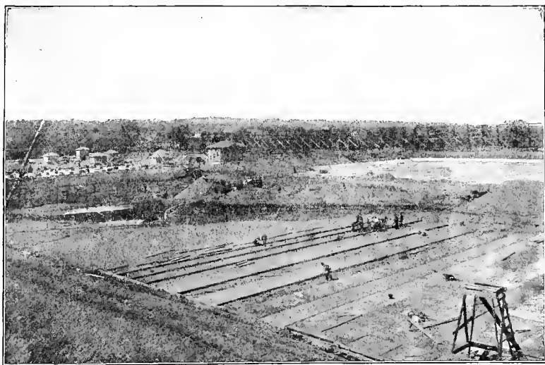
SEDIMENTATION-BASIN : SHOWING CONSTRUCTION OF FLOOR.
